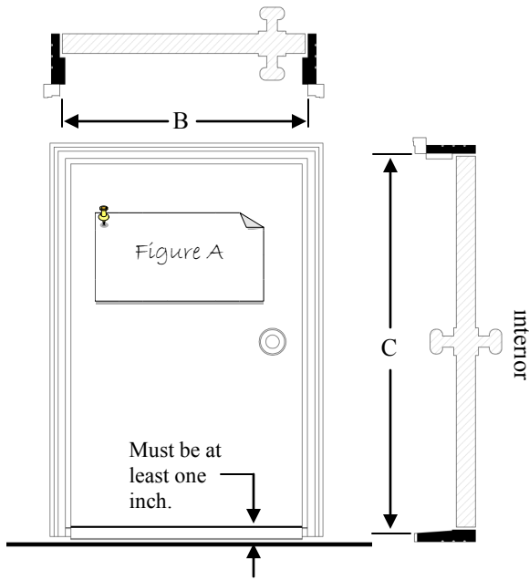
Outswing Door—Inside mount
