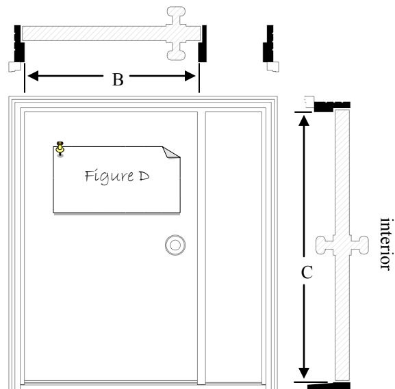
Inswing Door with Side Light mount
