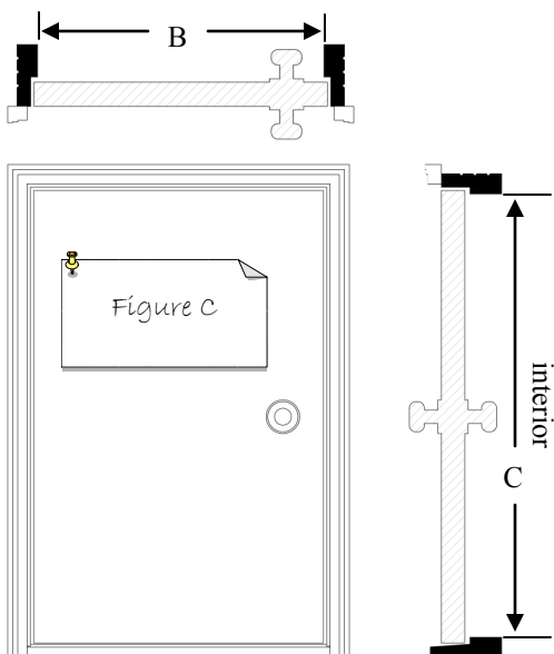
Outswing Door—Inside mount
