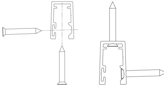
Showing screw clearances on track mounts
